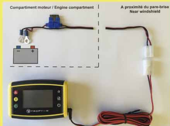
Porte fusible automobile / Automotive fuse holder
